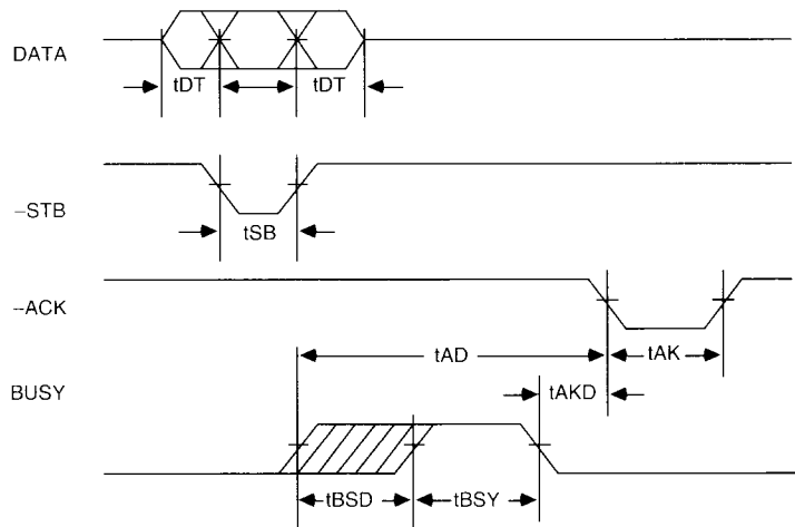
FIGURE 16.
