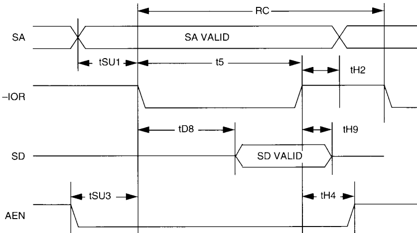
FIGURE 7. READ CYCLE
