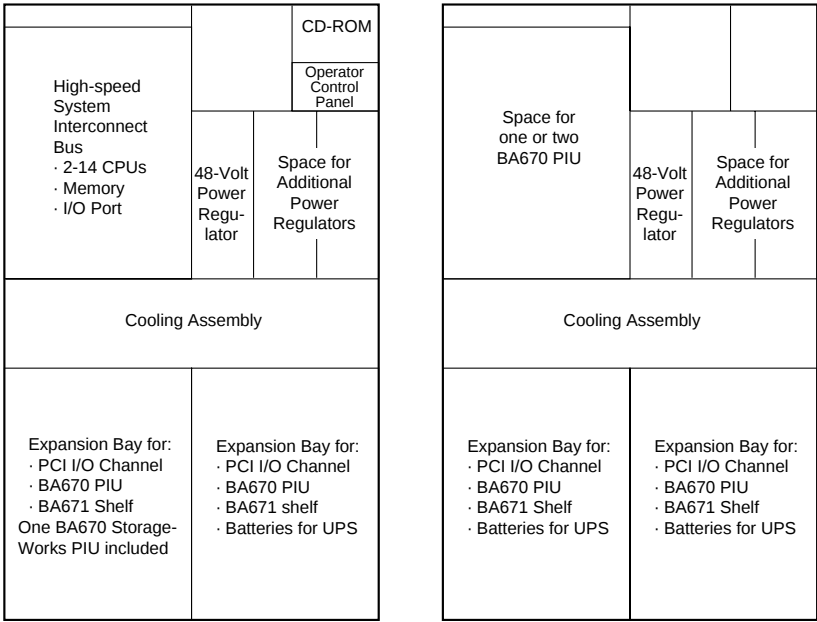
System Cabinet
