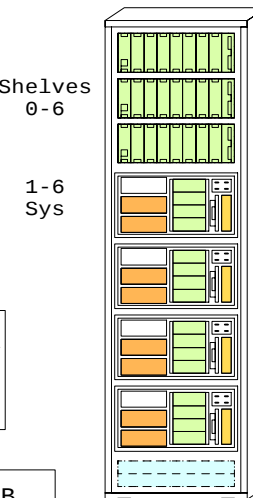
AlphaServer DS20E in Cabinet H9A15
